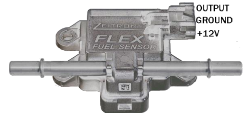
Flow Through Flex Fuel Sensor Pinout Image for reference only
